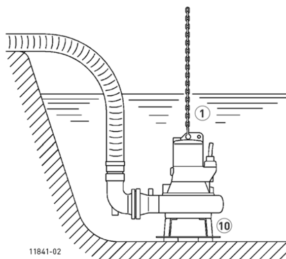
Example of installation pump base
