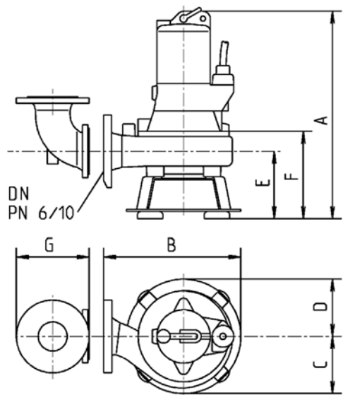
Dimensions pump base
