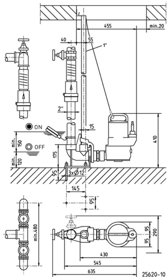
Dimensions with GR 50 (mm)
