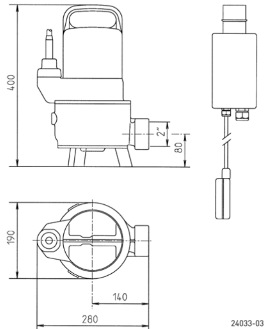
Dimensions US 253 (mm)
