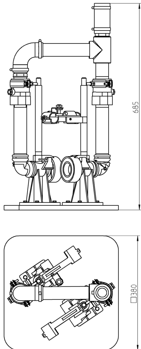
Dimensions Easyfix 32 Duo (mm)
