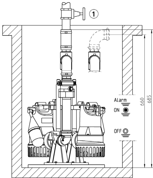
Example of installation Easyfix 32 Duo
