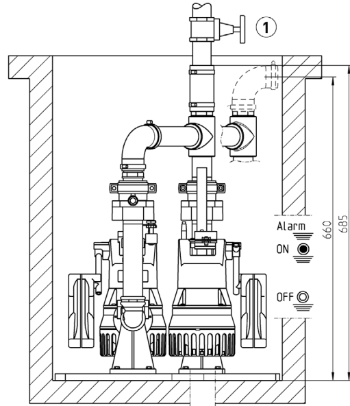
Example of installation Easyfix 32 Duo with special float
